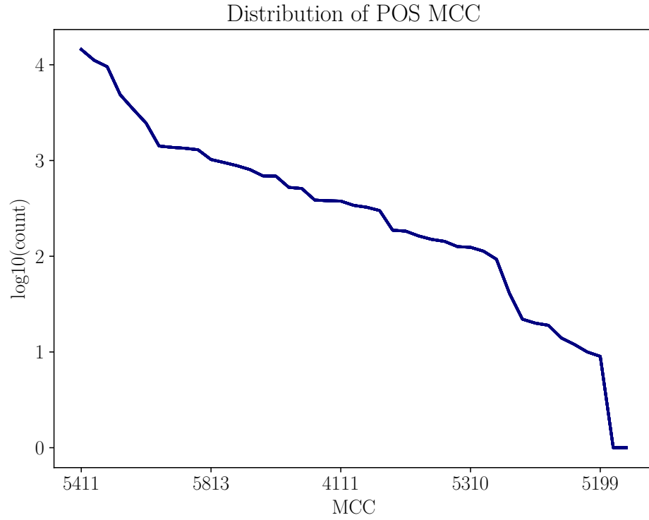
Figure 4.4: Distribution of POS MCC.
